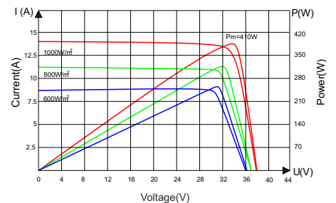
Current-Voltage&Power-Voltage Curve(410W)
